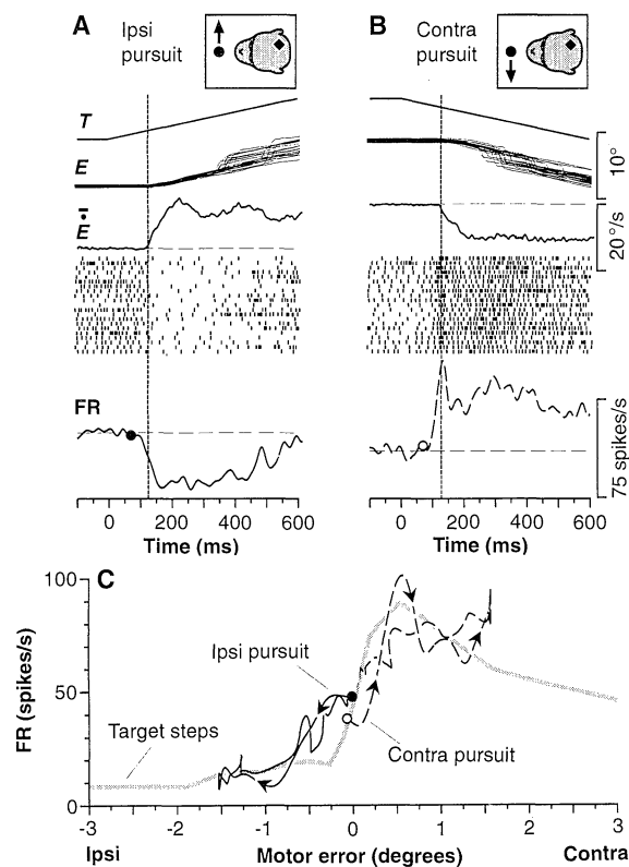
Fig. 2. Response of a neuron in the rostral SC during pursuit eye movements of a ramp target motion. (A) and (B) Activity of a neuron (1 from Fig. 1) shown during pursuit directed toward the ipsilateral (ipsi) (A) or contralateral (contra) (B) side. Within each panel, the stack of records shows the target position ( T ), the superimposed eye position traces from each trial ( E ), the average eye velocity across all trials ( \bar{E} ), a raster display of the neuronal responses, and the average firing rate (FR) shown as a spike density function (using a Gaussian curve with \sigma = 10 ms). Records are aligned on the onset of target motion (10°/s ramp), which is defined as time zero; vertical lines indicate the onset of pursuit. (C) The firing rate of neuron 1 recorded during pursuit as a function of the motor error 70 ms before. Different line types plot the firing rates during ipsiversive (solid line) and contraversive (dashed line) pursuit. Filled and open circles indicate the start of the two curves, corresponding to the firing rate at 70 ms after the onset of target motion. Arrows placed along the curves indicate increasing time. For clarity, arrows are placed only on data from the first half of the trial, when the motor error was increasing. The gray curve is as in Fig. 1C.
