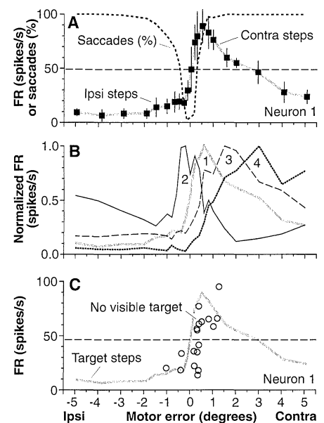
Fig. 1. Tuning of neurons in the rostral SC for small mismatches between eye and target positions. (A) Modulation in the firing rate (FR) of neuron 1 recorded after small ipsiversive (ipsi) and contraversive (contra) steps of a target presented on a homogeneous background. Square symbols plot the average firing rate from 12 trials over an interval beginning 100 ms after the step and lasting either 100 ms or until 8 ms before any corrective saccade. Error bars indicate \pm 1 SD. Dotted line indicates the percentage of trials in which each amplitude of the target step elicited a saccade. Saccades were detected as any eye movement exceeding 5°/s and 800°/s 2 ; these criteria identified saccades as small as 0.05°. Dashed line indicates the average firing rate with no target steps. (B) Modulation of four rostral SC neurons (numbers 1 through 4) after small steps; all were recorded from the right SC of one monkey. The data have been normalized so that the peak of each curve equals 1. (C) Firing rate of neuron 1 recorded as the monkey maintained fixation after the visual stimulus was extinguished. Circles indicate the average firing rate during each of 18 saccade-free intervals lasting 73 to 230 ms and are plotted as a function of the average motor error during each interval. Dashed line indicates the average firing rate across all intervals. The superimposed gray curve shows the discharge of the same neuron when the stimulus was still present, as in (A).
